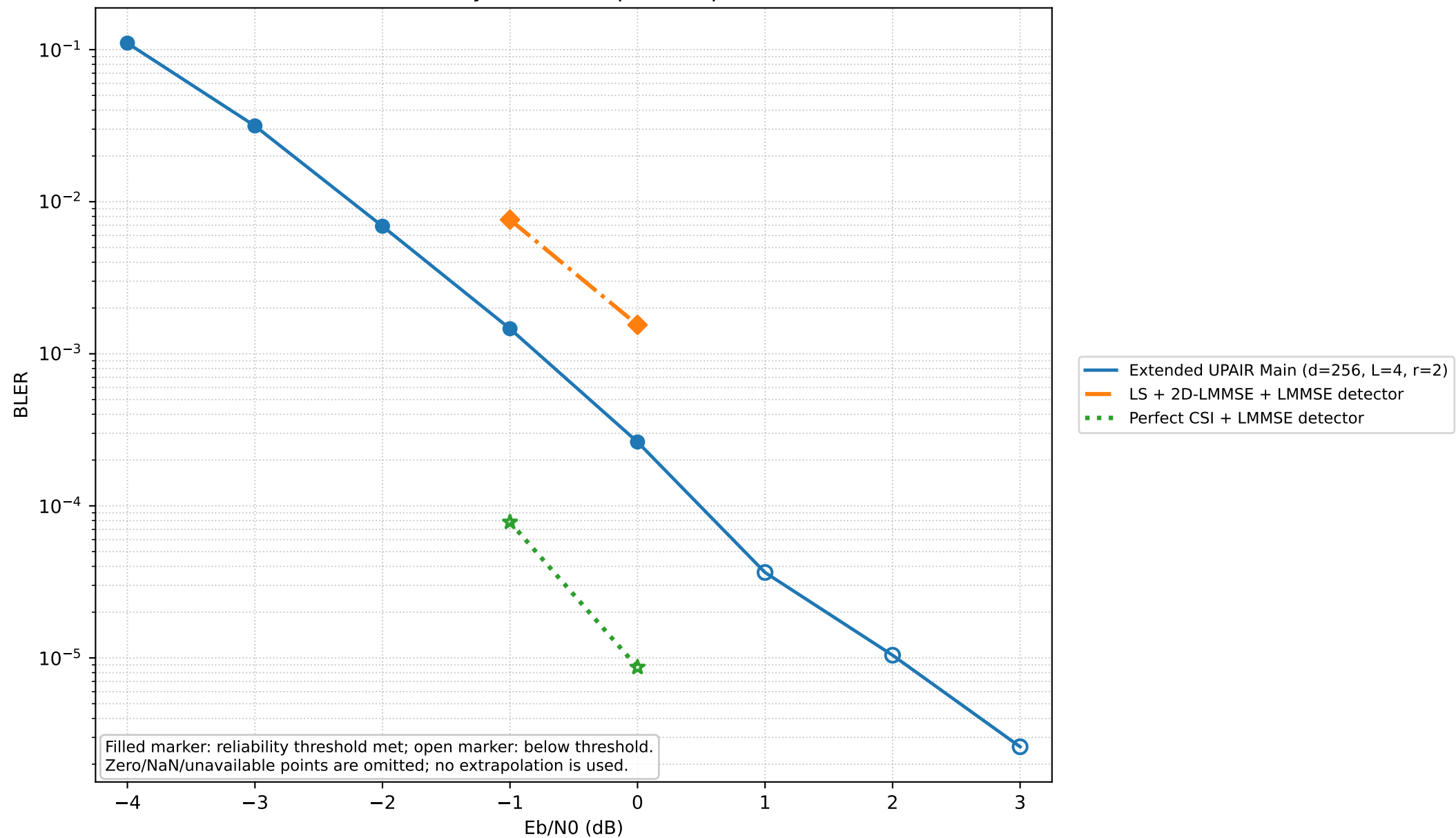
Extended UPAIR Main (d=256, L=4, r=2) vs Available Benchmarks — BLER 3 active users — only evaluated, positive points are shown
